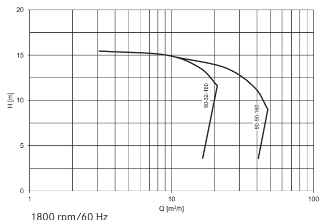
1800 rpm/60 Hz
