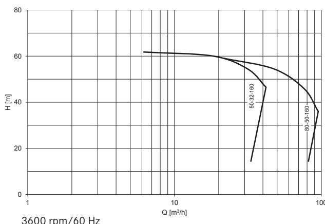
3600 rpm/60 Hz
